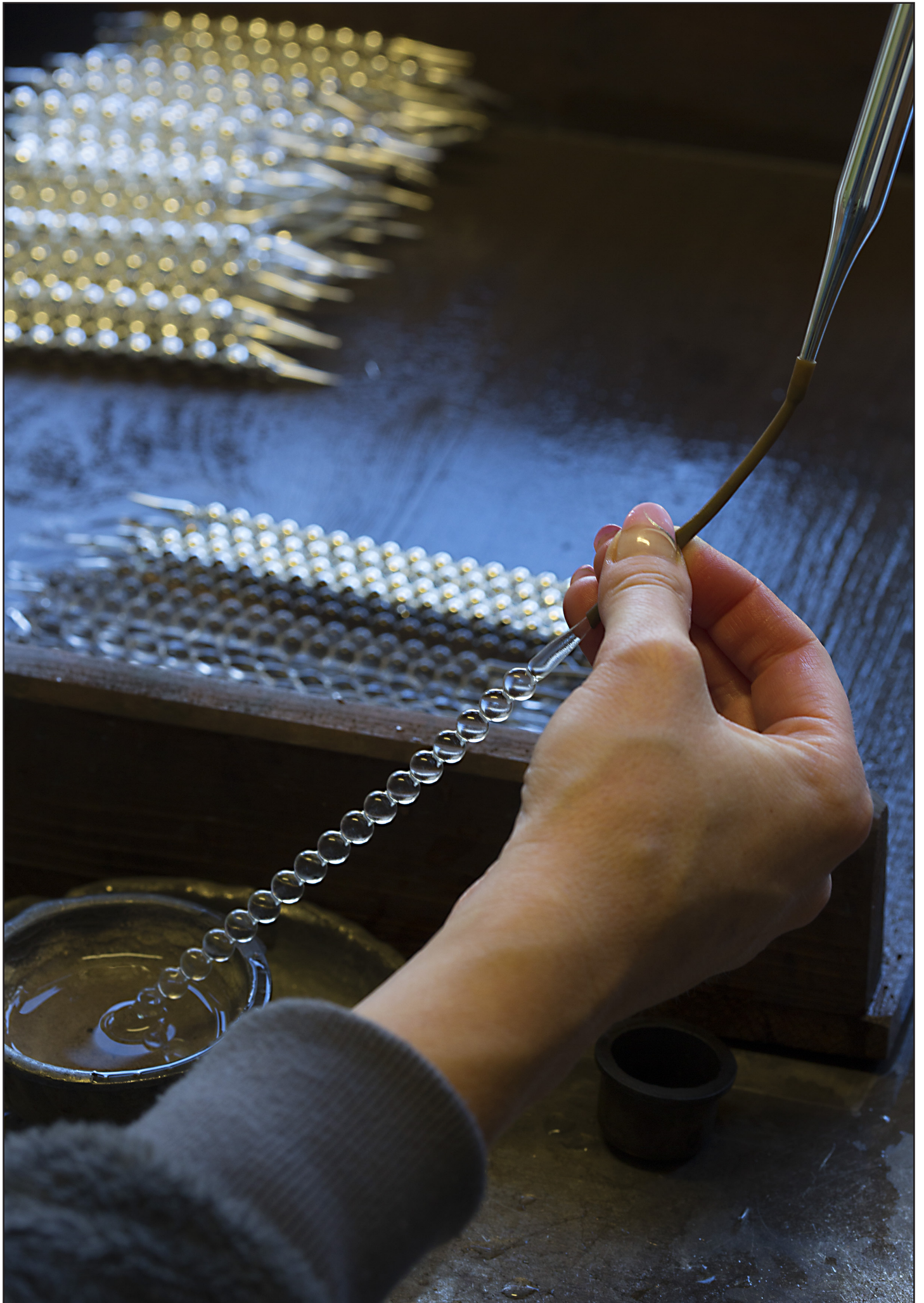
Photo no. 5 Hand made Production of Christmas Tree Decorations from blown glass Beads; silvering
